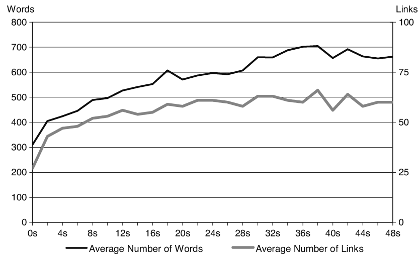
Fig. 5. Correlation between stay time, page contents and link count.
