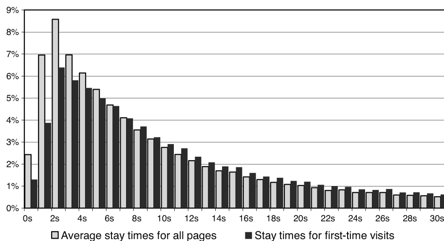
Fig. 4. Distribution of stay times for all participants.
