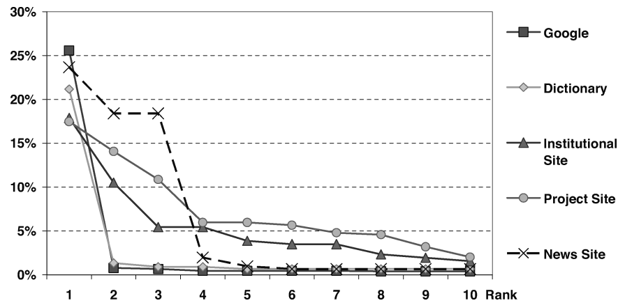
Fig. 7. Distribution of page revisits for different categories of Web sites.
