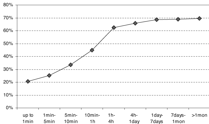
Fig. 2. Proportion of changed pages for different revisitation periods.
