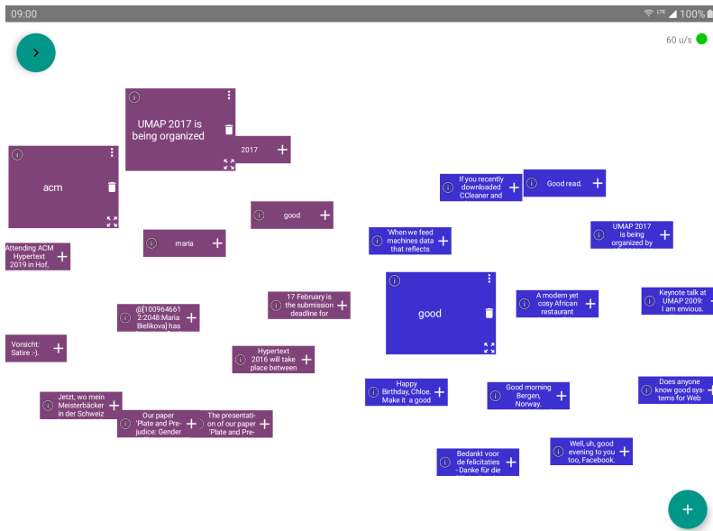
Fig. 2: Screenshot of the prototype. One post and two keywords are added. Related entities surround the selected posts and words by means of attraction and repulsion, and two spatial clusters are created based on content similarity.
